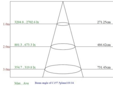
LUX Diagram
