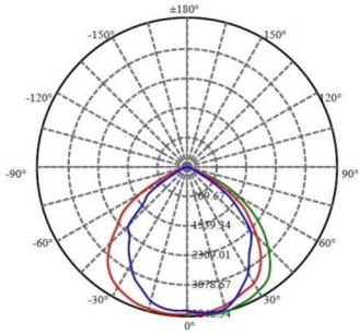
Radiation Diagram
