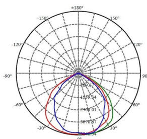
Radiation Diagram
