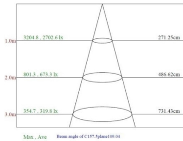
LUX Diagram
