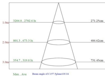
LUX Diagram
